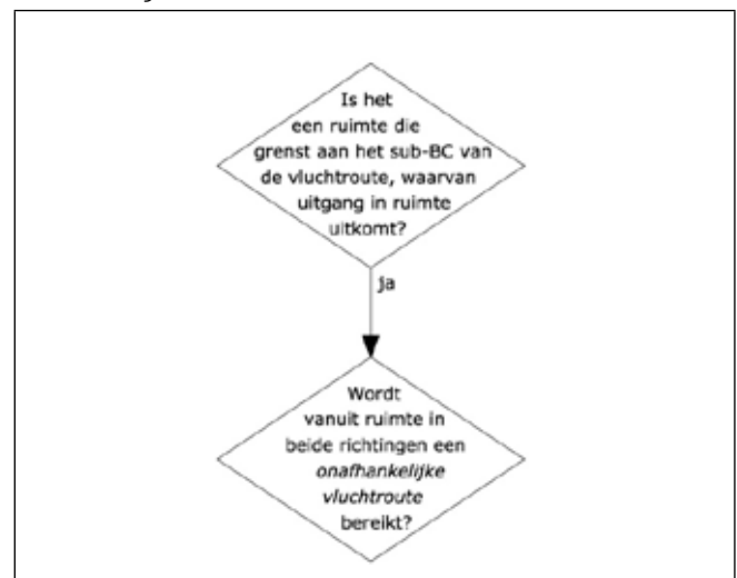
Stroomschema 3d.C
